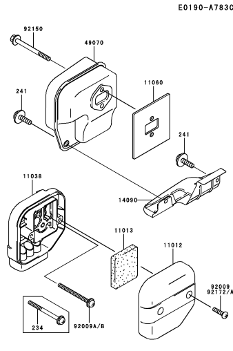
B-10 AIR-FILTER/MUFFLER
