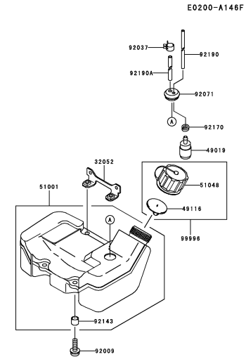
B-11 FUEL-TANK/FUEL-VALVE
